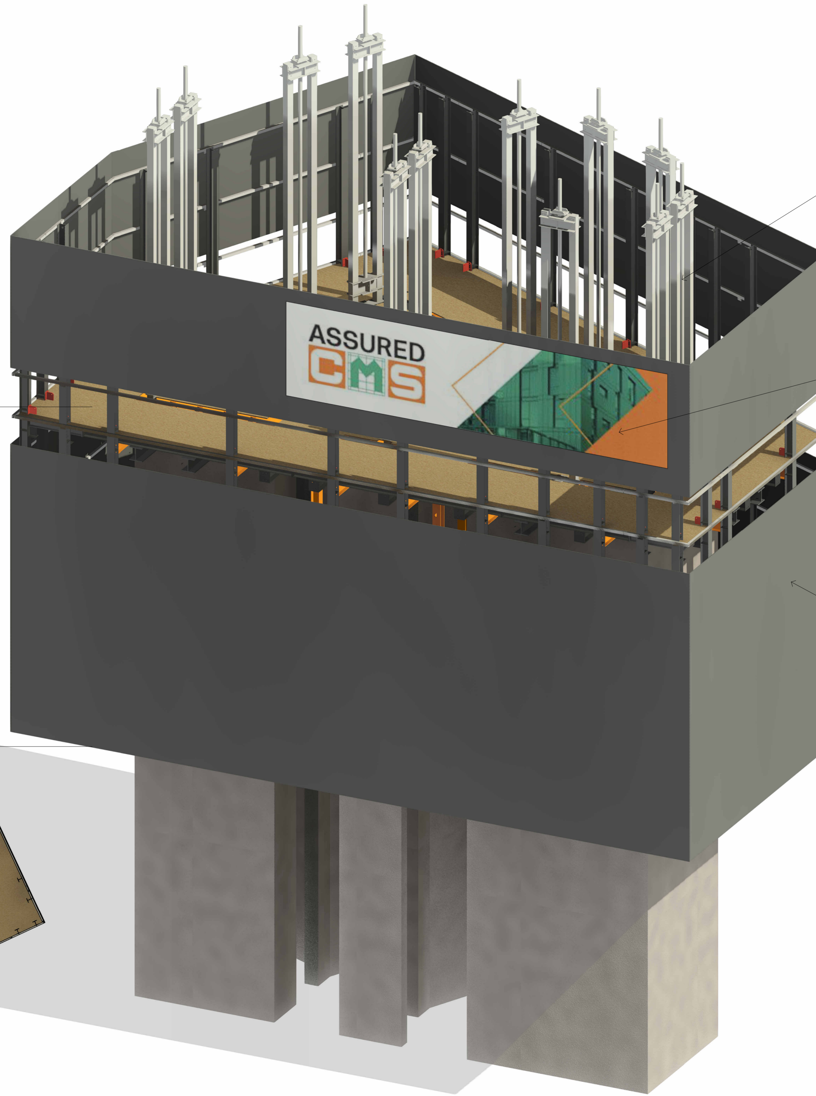
JUMPFORM 3D VIEW
