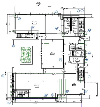
1 - FIRST FLOOR PLAN
