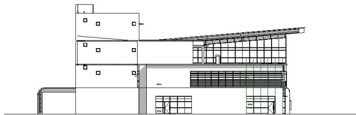
1 - WEST ELEVATION 1/8" = 1'-0"
