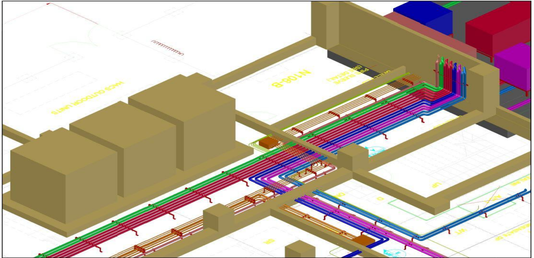
COMBINED SHOP DRAWING OF MECHANICAL REFRIGERANT LIQUID AND GAS AND ELECTRICAL CONDUITS AND CABLE WIRES
