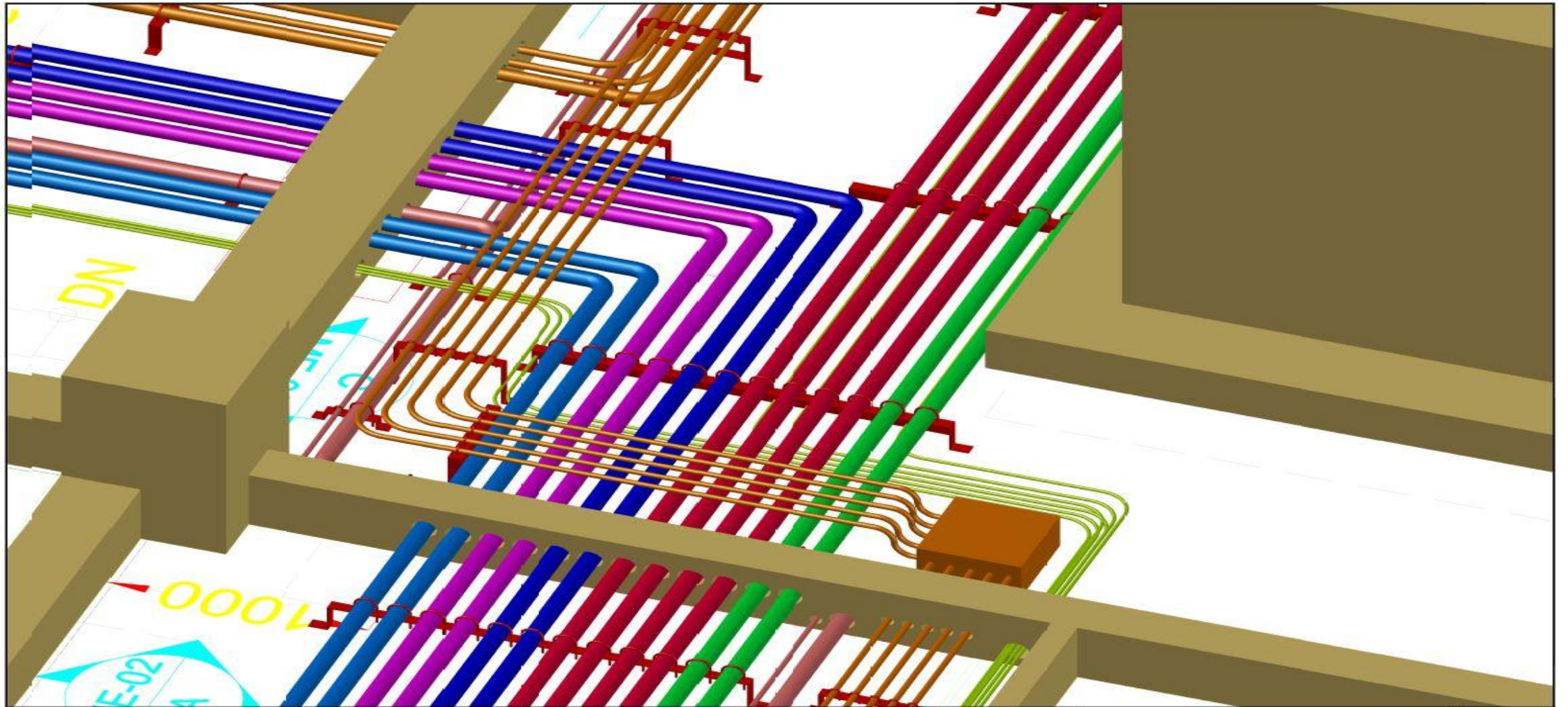
COMBINED SHOP DRAWING OF MECHANICAL REFRIGERANT LIQUID AND GAS AND ELECTRICAL CONDUITS AND CABLE WIRES
