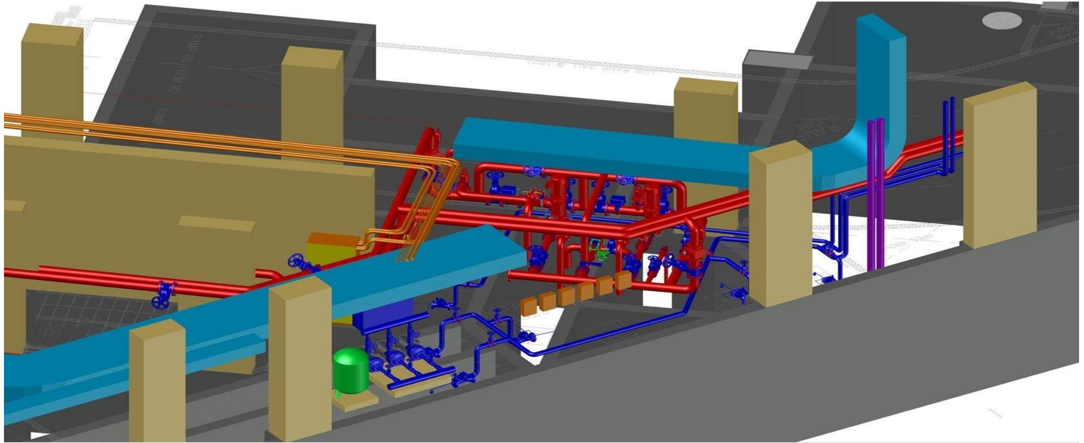
COMBINED SHOP DRAWING OF MEPPS AT PUMP ROOM (3D)
