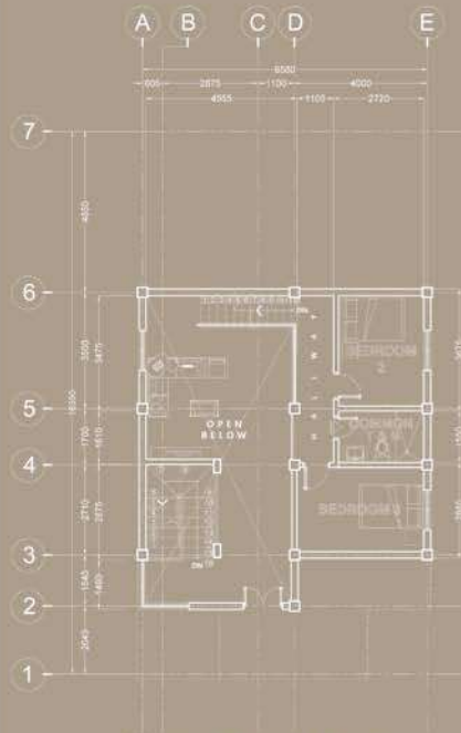
2 LOFT FLOOR PLAN A2 SCALE 1:100m
