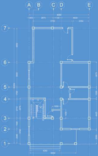
2 PROPOSED GROUND FLOOR PLAN A1 SCALE 1:100m
