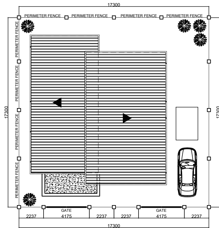
A 23 SITE DEVELOPMENT PLAN SCALE 1:200 MTS
